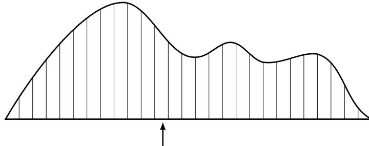
Figure 4: Physical interpretation of expected value as the balance point.
